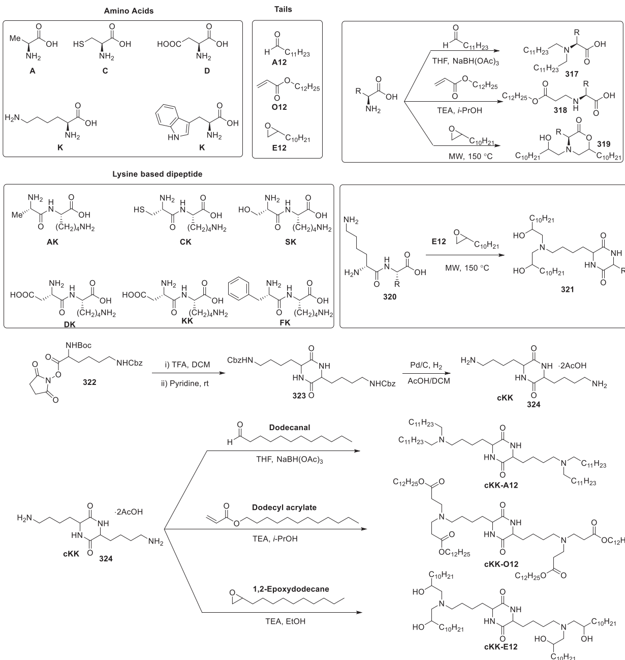
Figure 62. Synthesis of amino acid-derived lipidoids.
