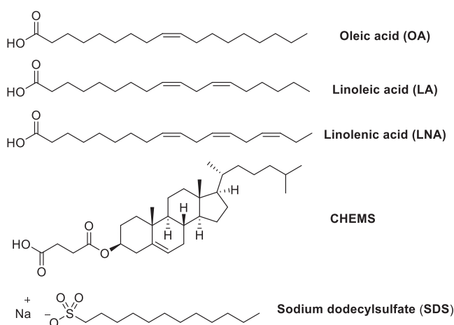
Figure 87. Chemical structures of anionic lipids.
