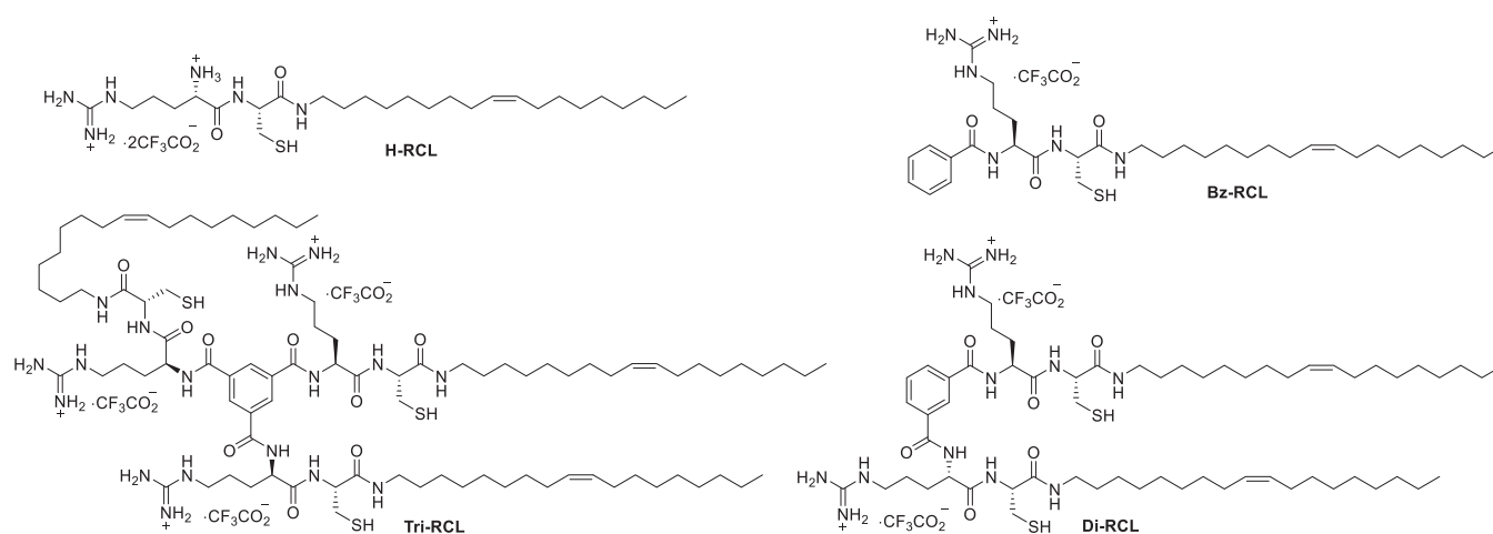
Figure 20. Chemical structures of arginine- and cysteine-derived guanidinium type lipids.
