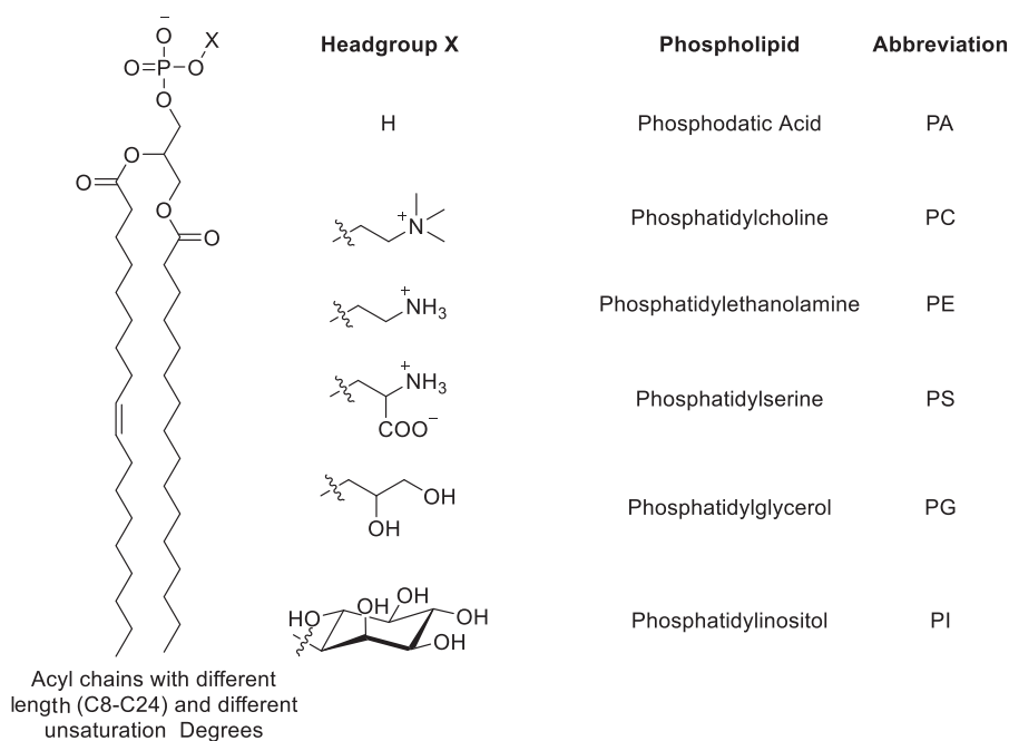
Figure 77. General chemical structure of phospholipids.
