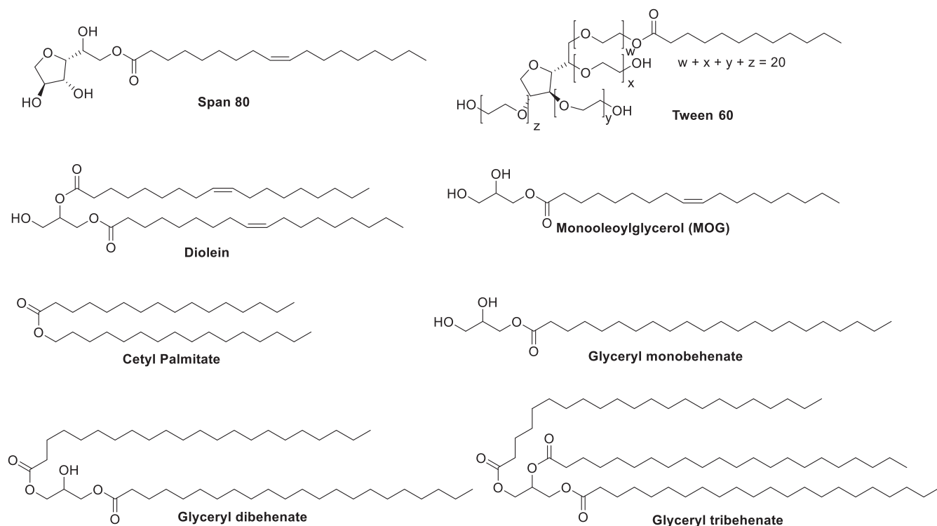
Figure 89. Chemical structures of fatty acid esters for RNA delivery.
