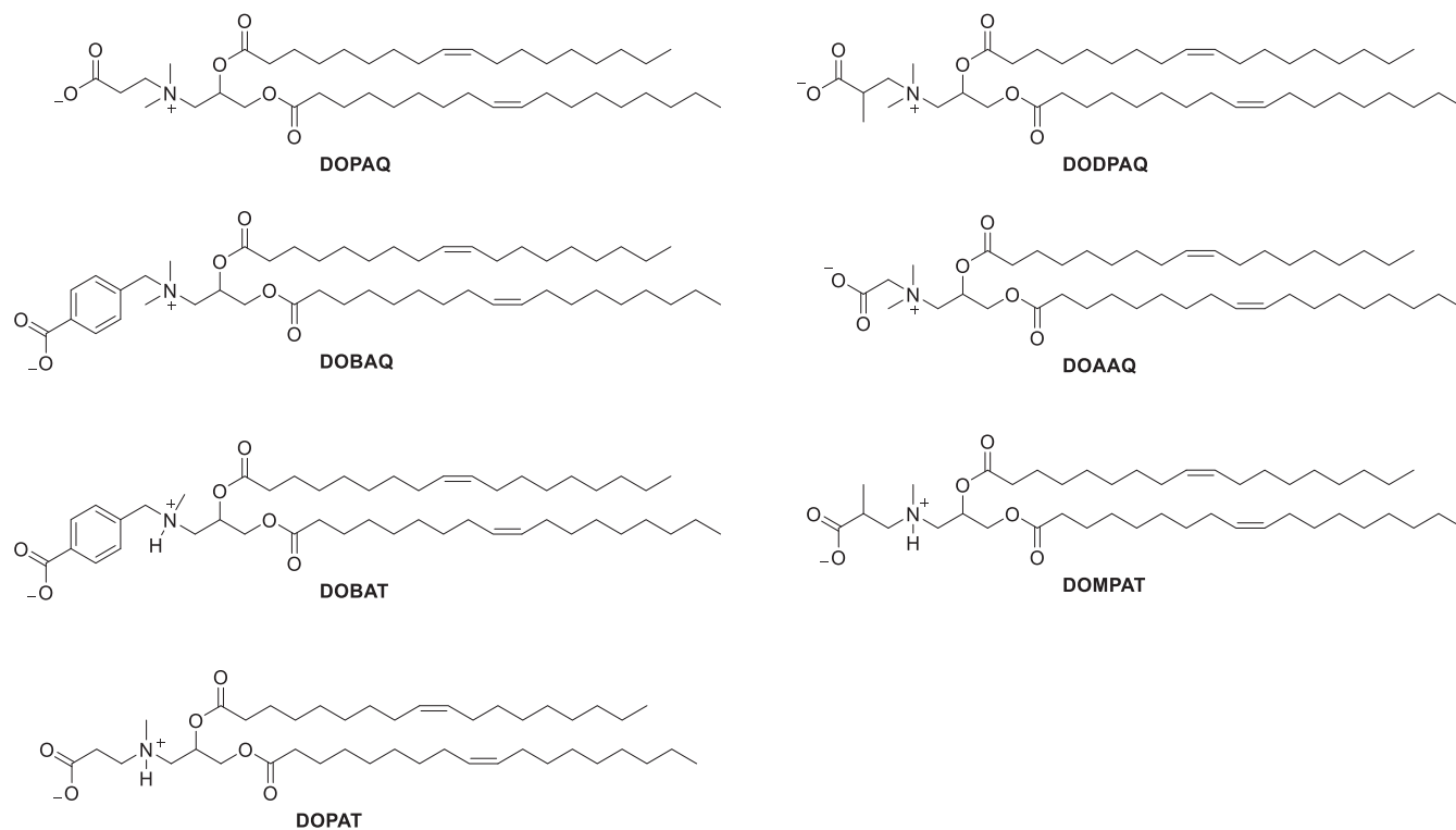
Figure 70. Chemical structures of zwitterionic lipids.
