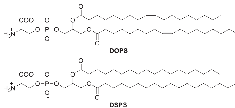
Figure 82. Chemical structures of representative phosphatidylserine.
