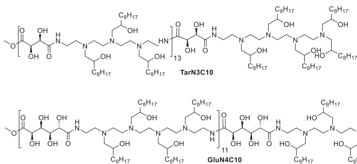
Figure 95. Chemical structures of other types of lipopolymers.
