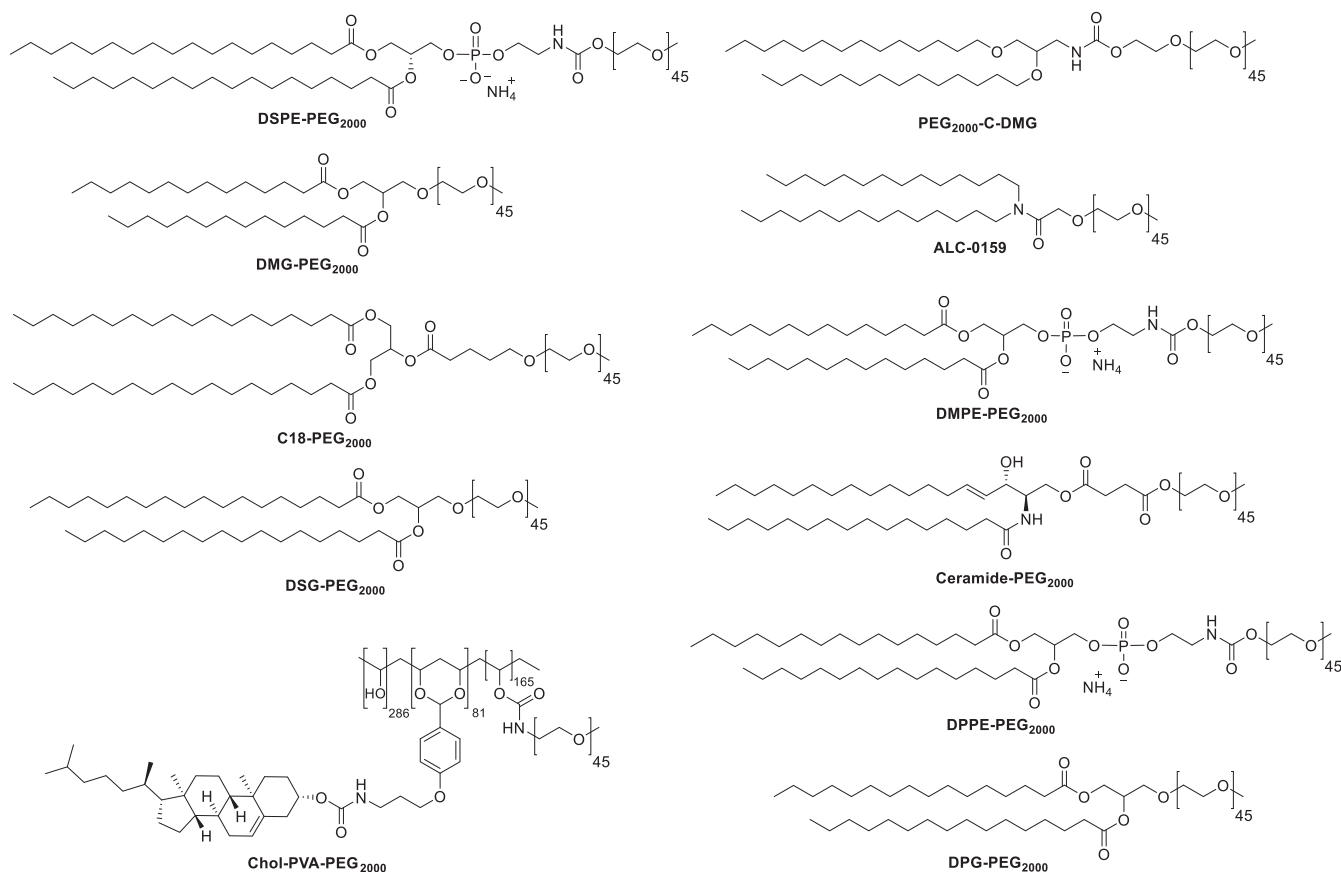
Figure 91. Chemical structures of PEG-lipids.
