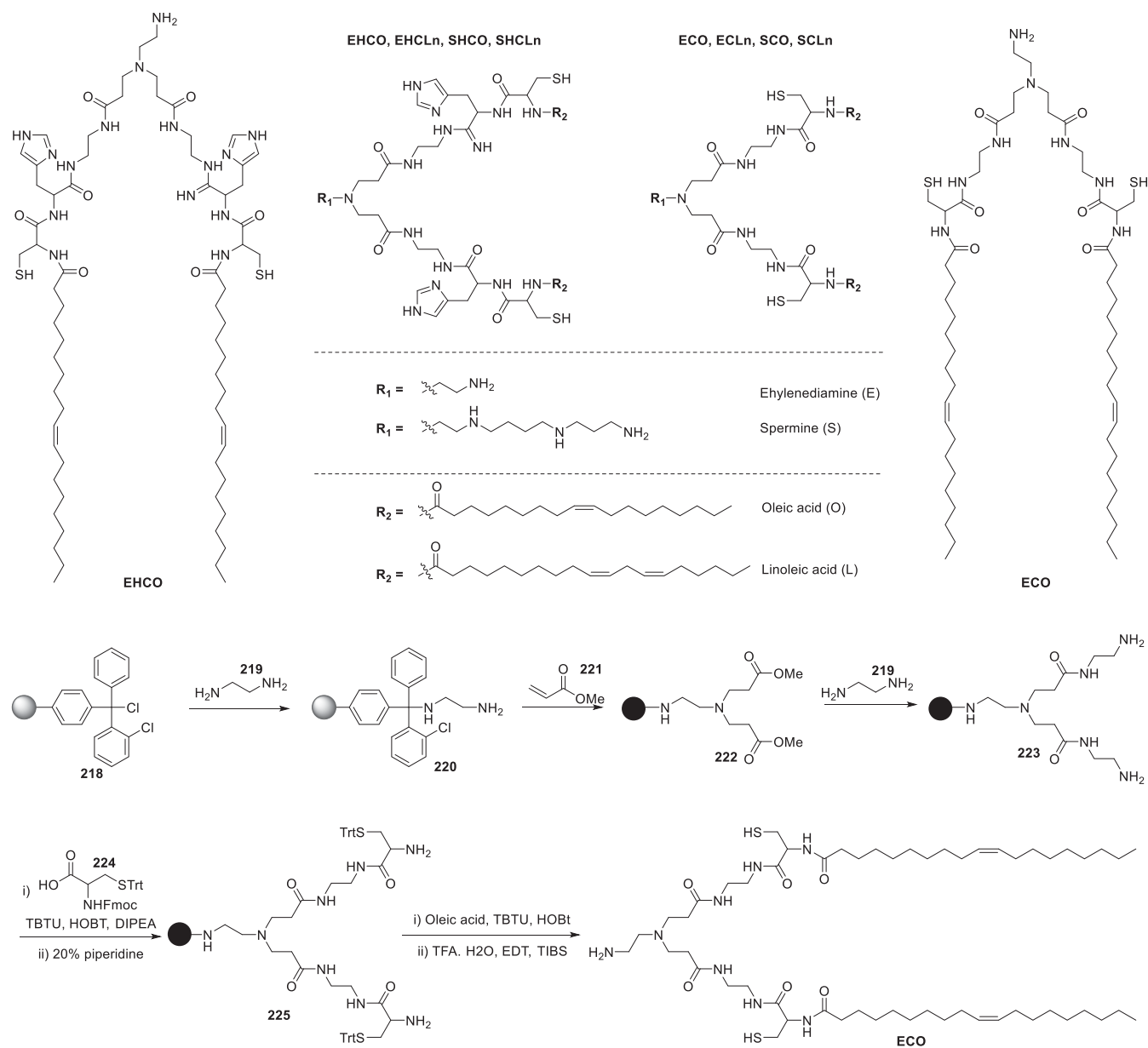
Figure 33. Chemical structures of multifunctional ionizable lipids.
