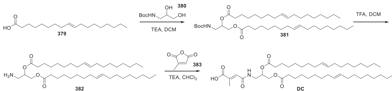
Figure 88. Synthesis procedures of DC.
