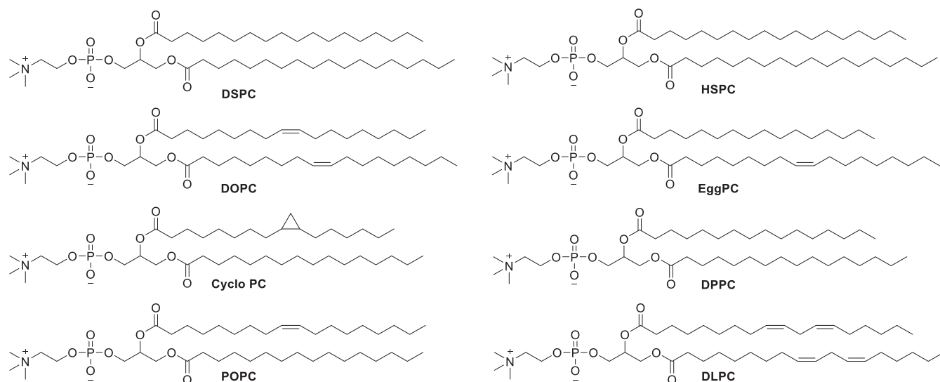
Figure 78. Chemical structures of representative phosphatidylcholines.
