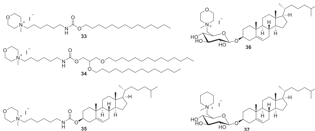
Figure 10. Chemical structures of piperidinium and morpholinium lipids.
