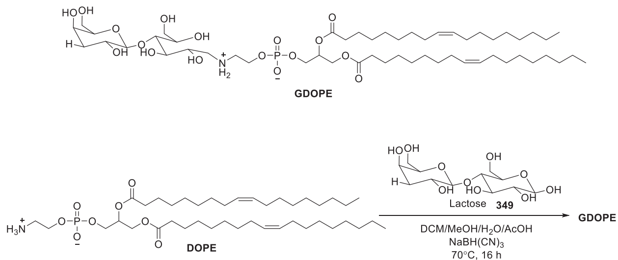
Figure 69. Chemical structure of zwitterionic lipid GDOPE.
