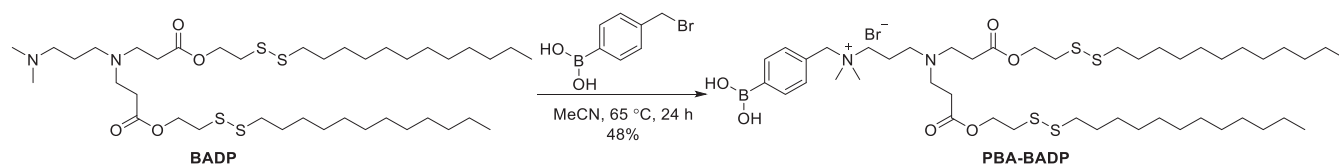
Figure 13. Chemical structure of PBA-BADP.
