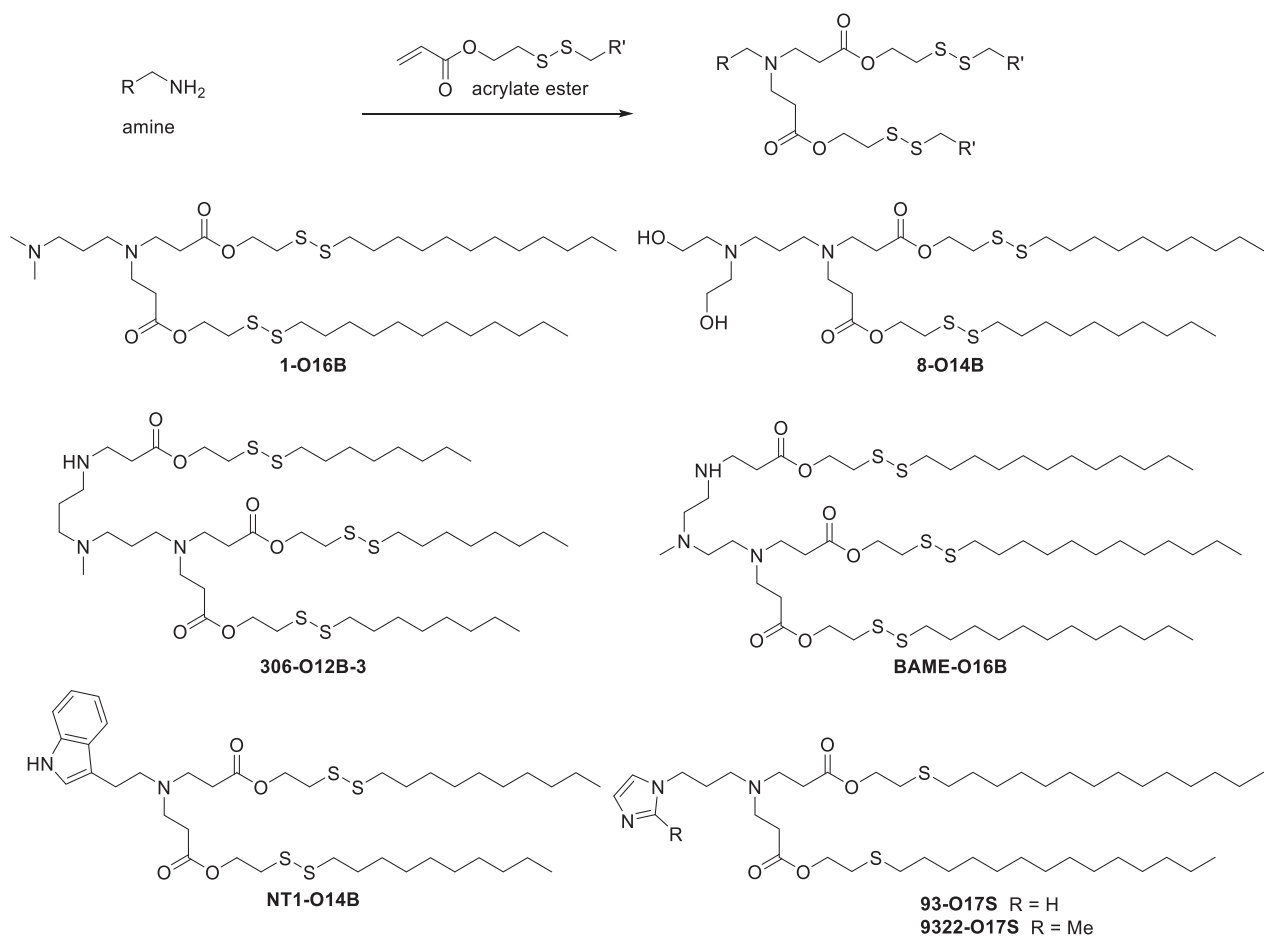
Figure 57. Chemical synthesis of bioreducible lipids.
