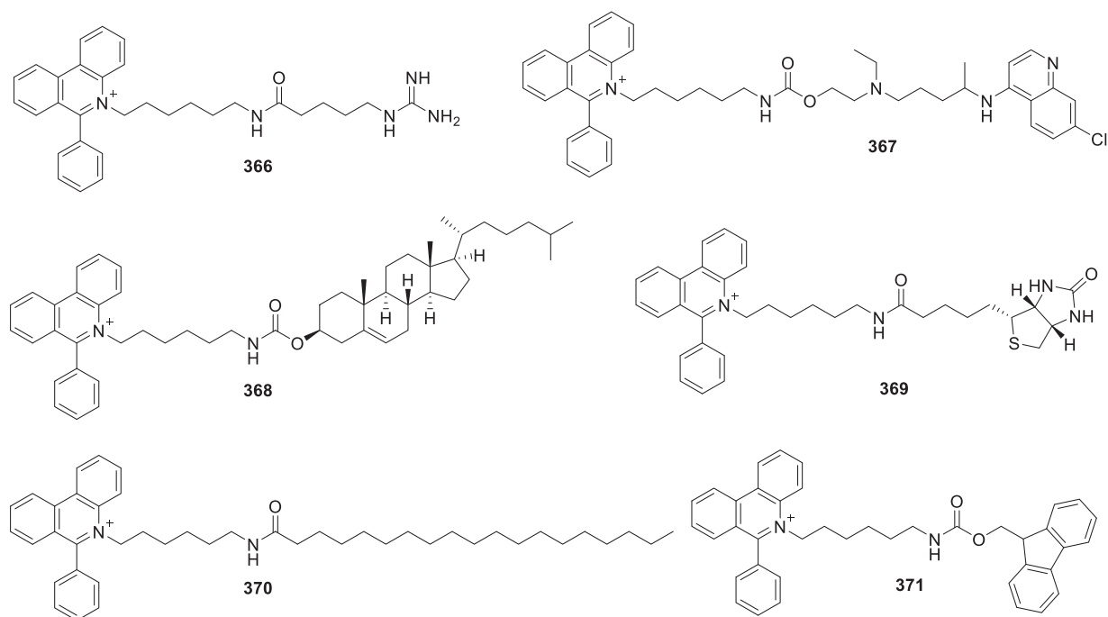
Figure 76. Chemical structures of representative coordinative amphiphiles (CAs).
