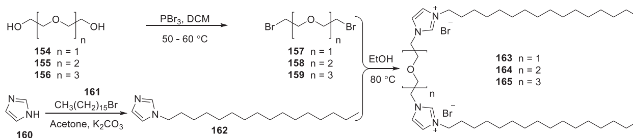
Figure 27. Synthesis of gemini imidazolium lipids 163–165.
