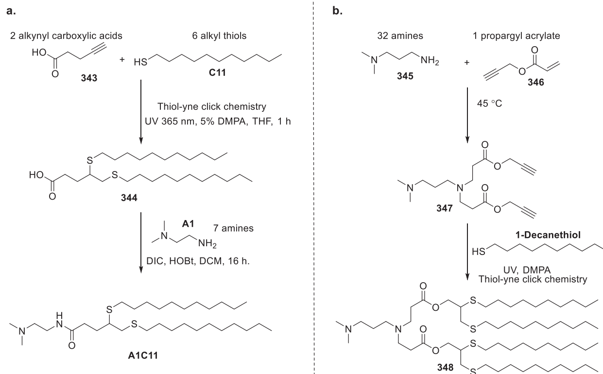
Figure 66. Synthetic routes to lipids via thiol–yne click chemistry.
