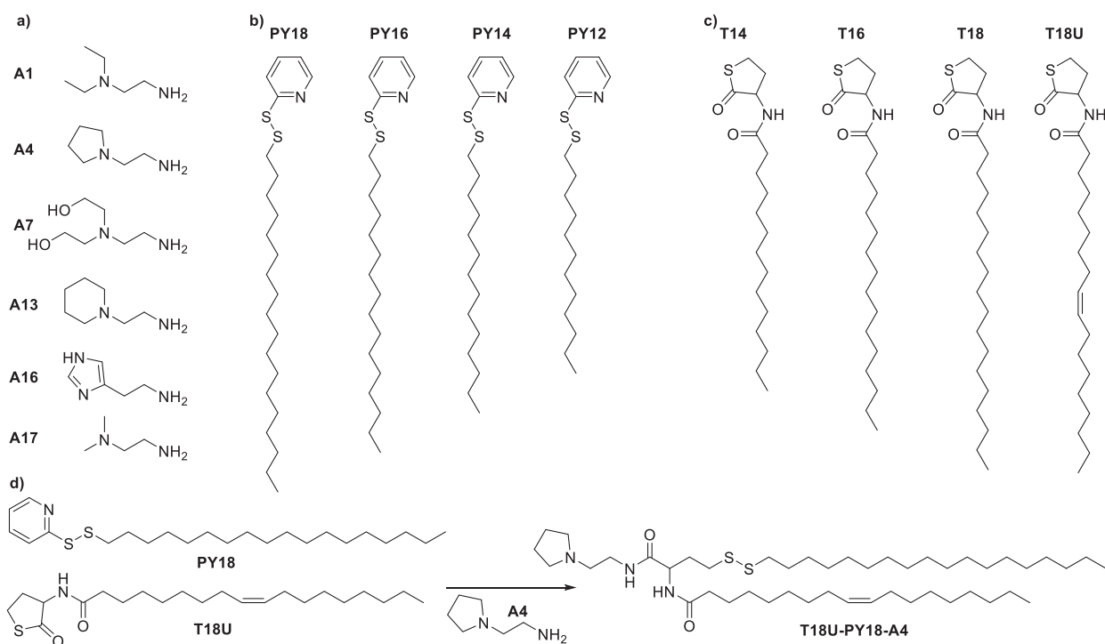
Figure 67. Synthesis of lipidoids via thiolactones ring-opening reaction followed by the thiol–disulfide exchange reaction. (a) Structures of amines. (b) Structures of pyridyl disulfide derivatives. (c) Structures of thiolactone derivatives. (d) Representative reaction scheme.
