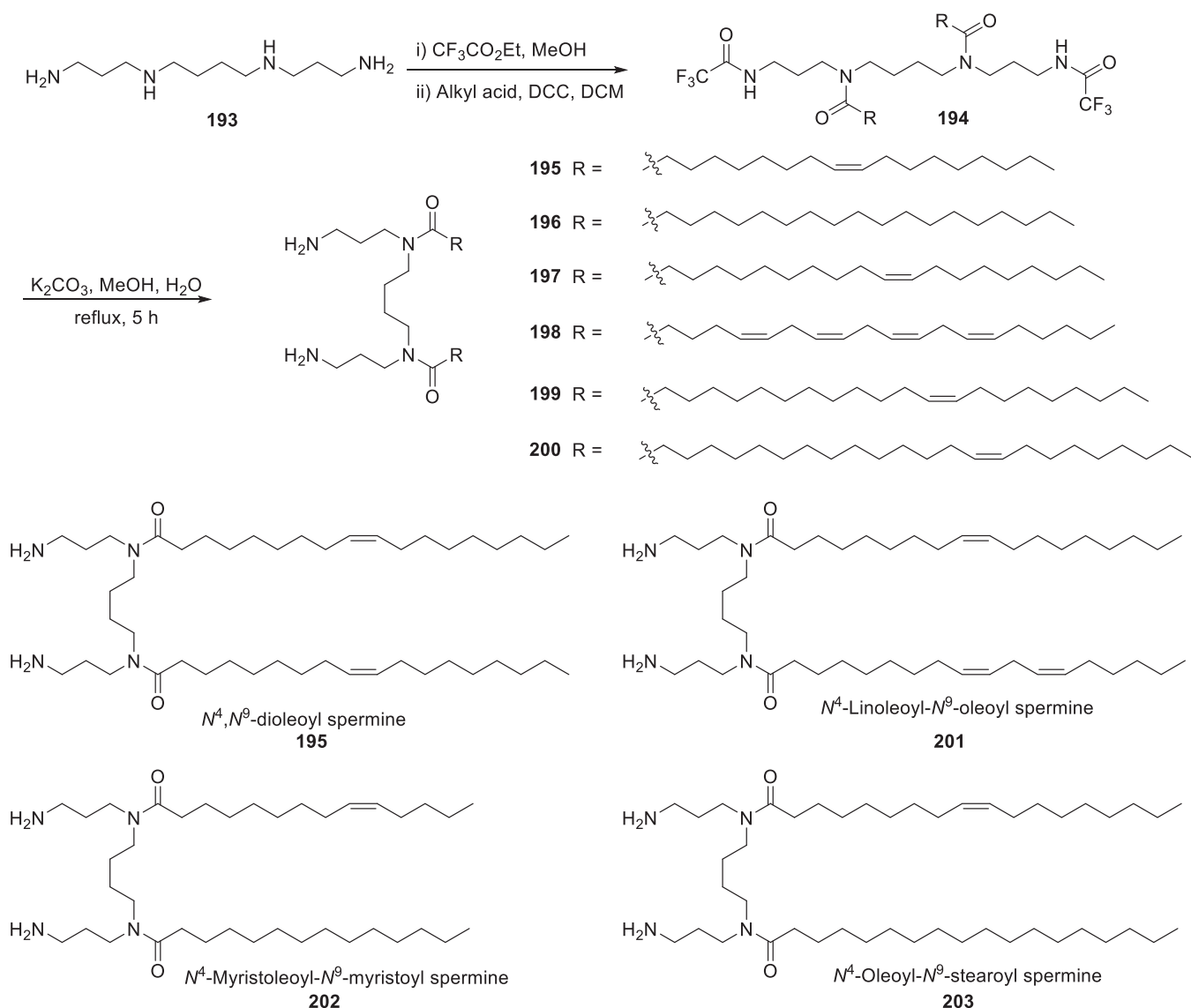
Figure 30. Synthesis of spermine-derived lipids.
