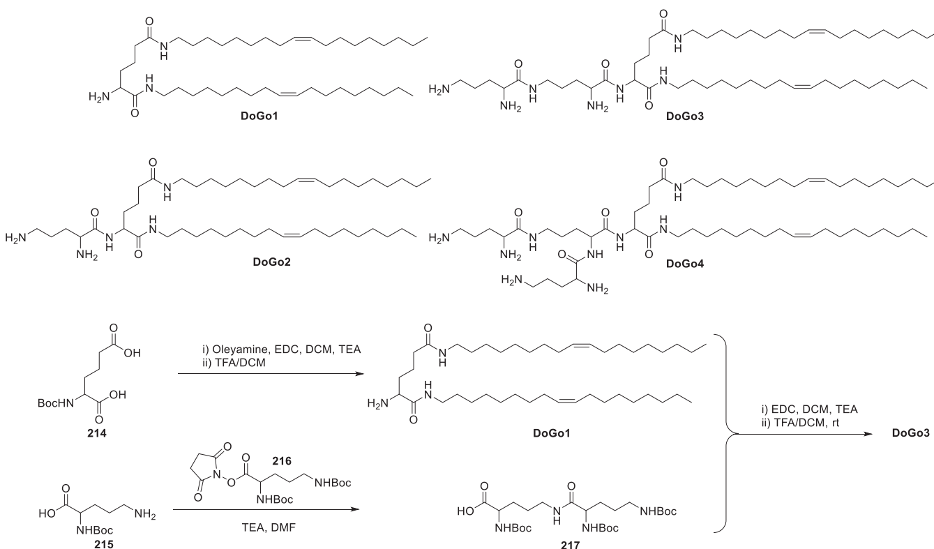
Figure 32. Chemical structure of lysine-derived lipids.
