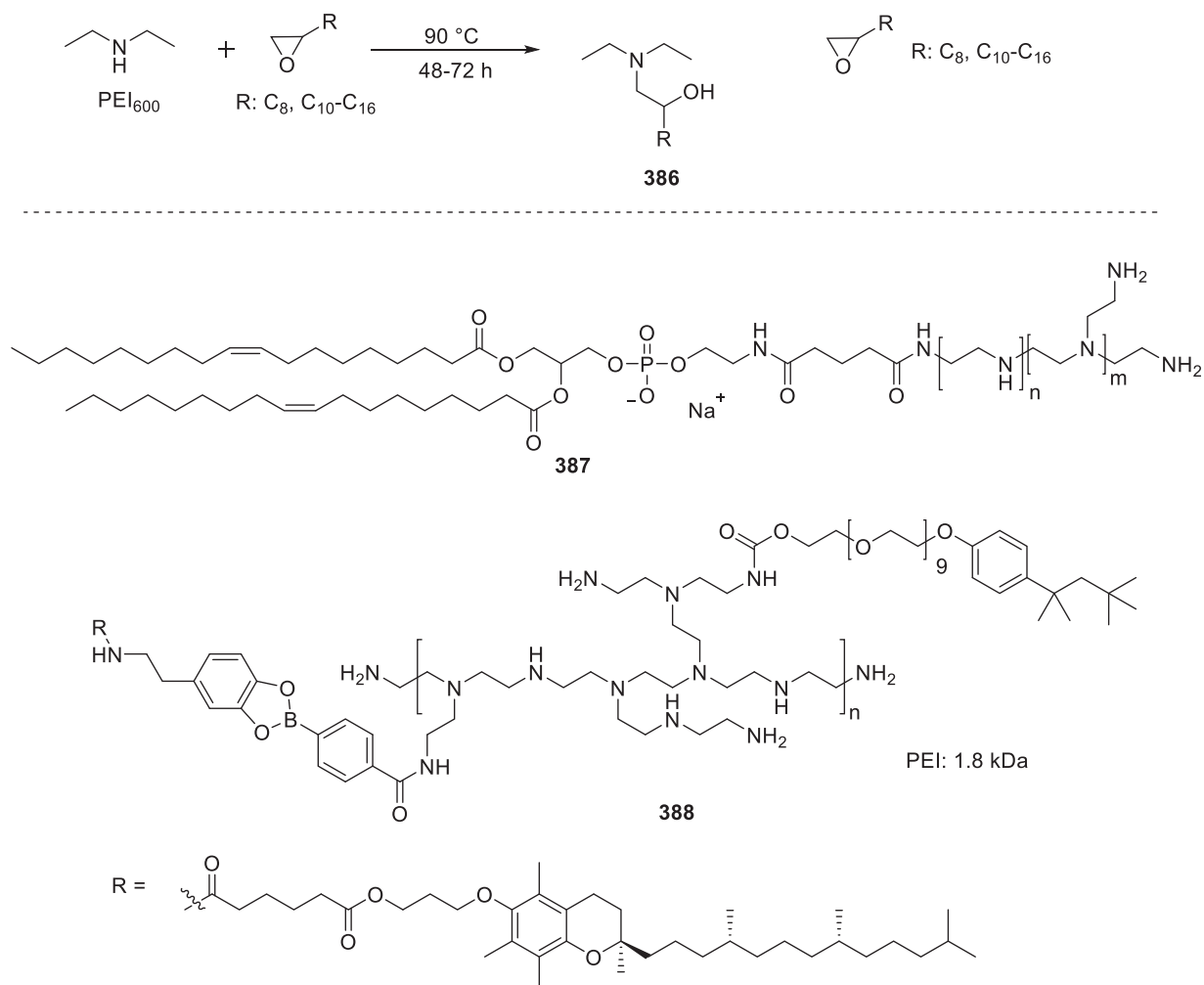
Figure 93. Chemical structures of PEI-lipids.
