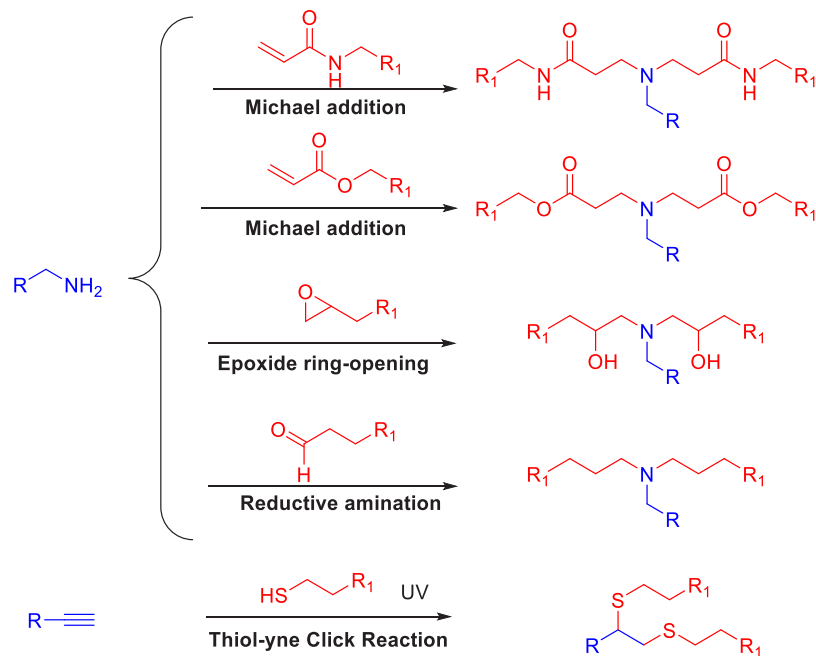
Figure 54. Representative reactions for the preparation of lipidoids.
