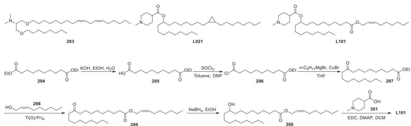
Figure 49. Chemical structures of lipid 293, L021, and L101 and a synthetic route to L101.
