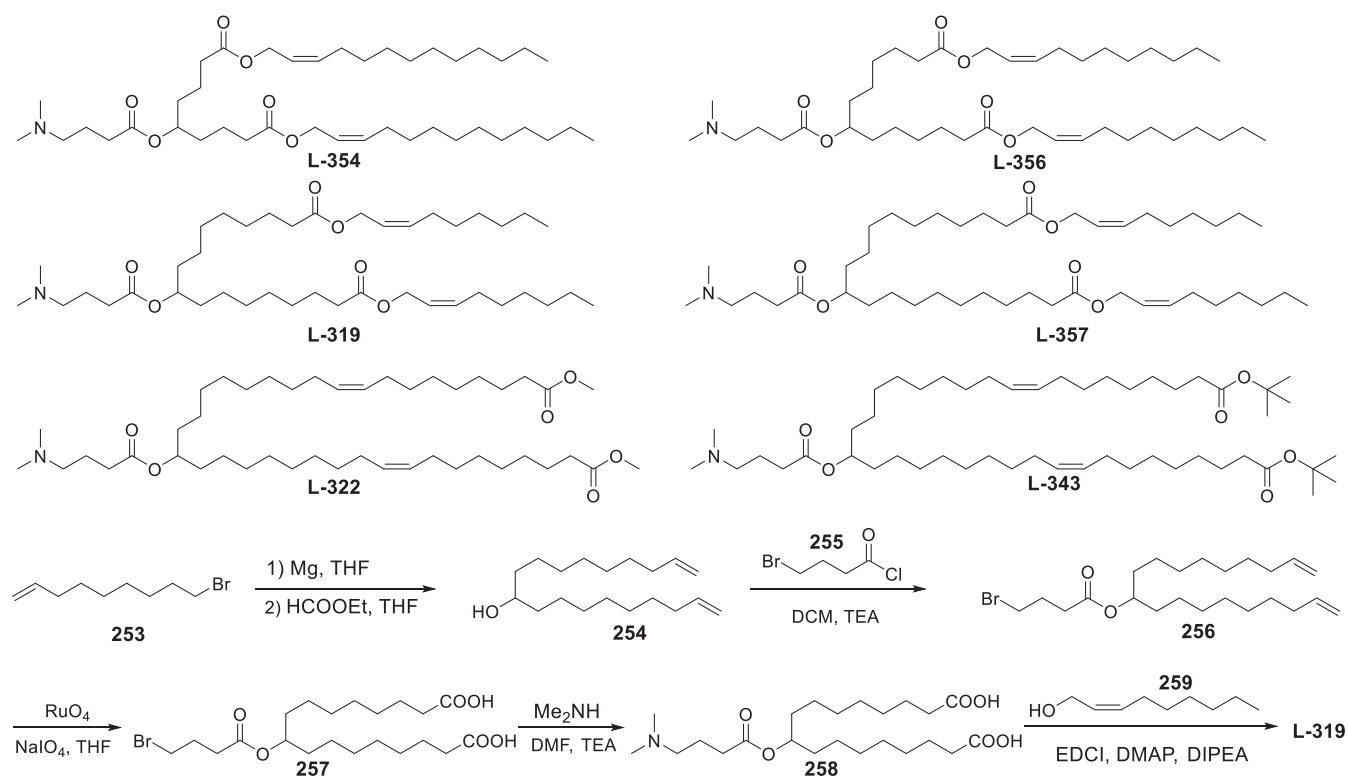
Figure 41. Synthesis of biodegradable dimethyl amino lipids.
