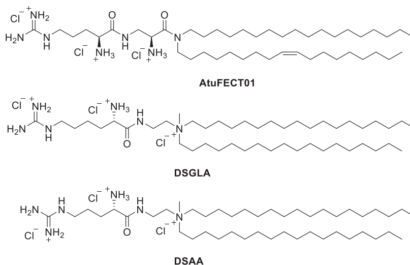
Figure 15. Chemical structures of AtuFECT01 and DSGLA.
