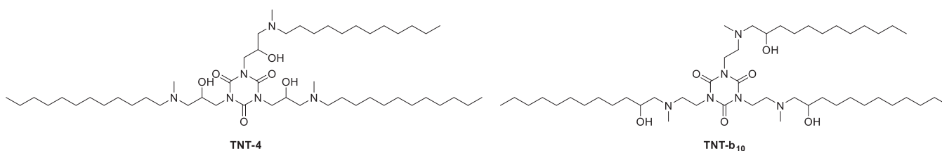
Figure 61. Chemical structures of TNT-4 and TNT-b 10 .
