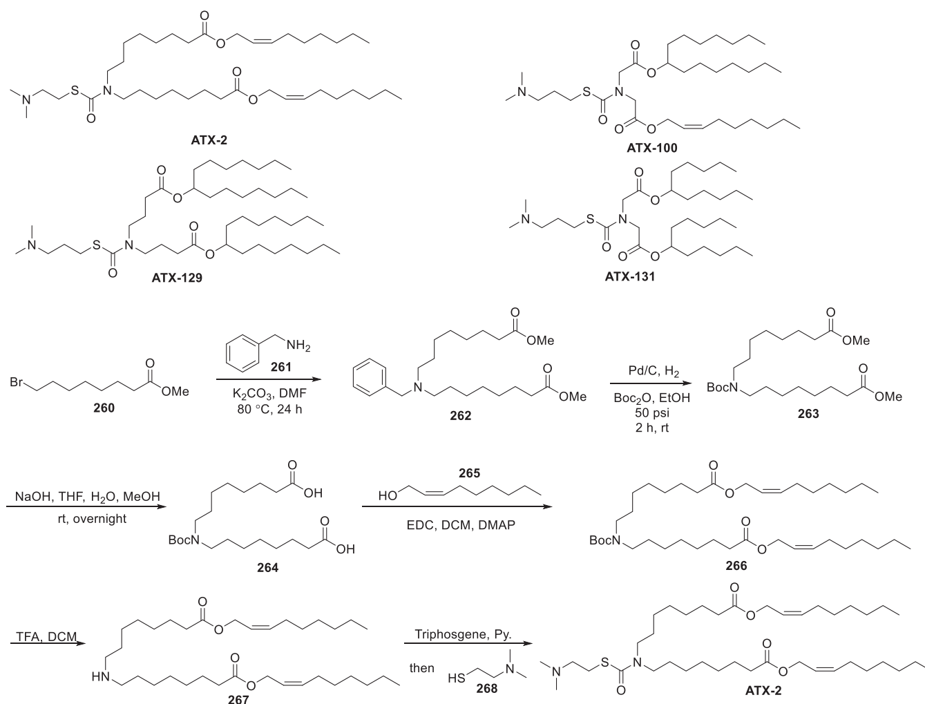
Figure 43. Chemical structures and synthesis of ATX lipids.
