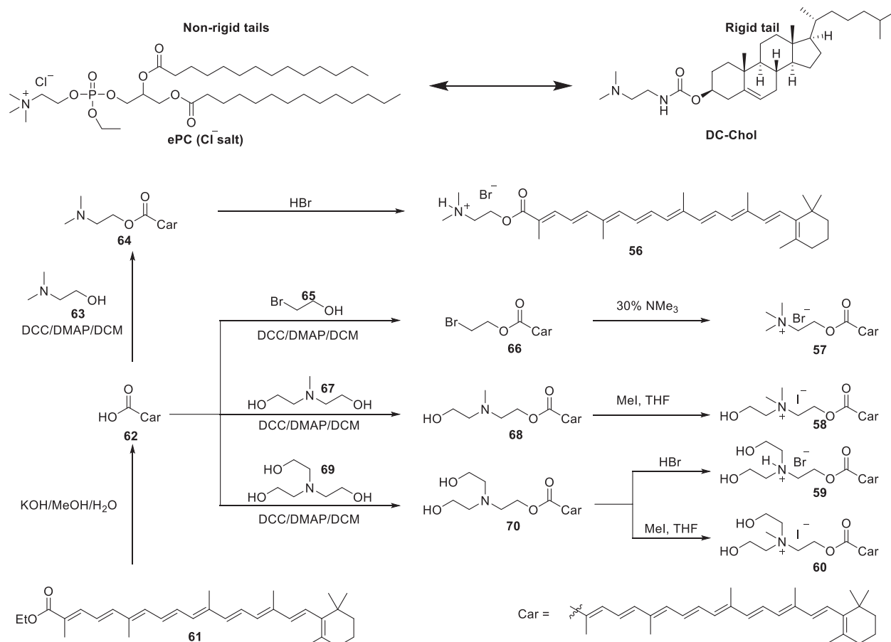
Figure 12. Chemical structures and synthetic route of carotenoid-derived lipids
