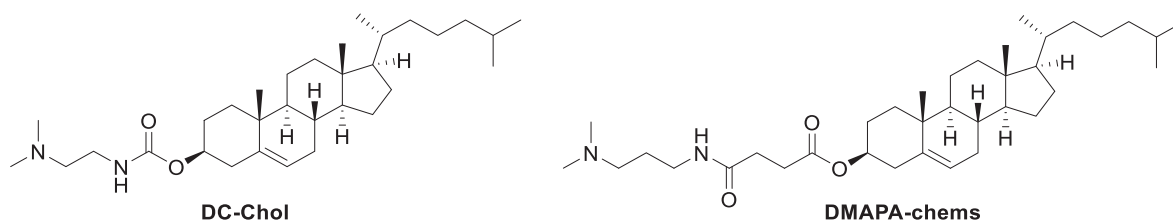
Figure 51. Chemical structures of cholesterol-derived ionizable lipids.
