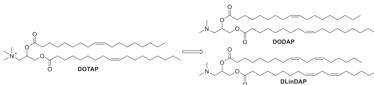
Figure 38. Chemical structures of DODAP and DLinDAP.
