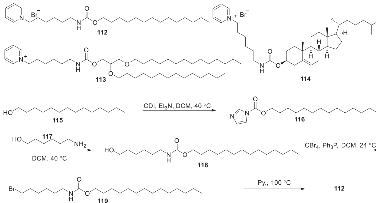
Figure 23. Chemical structures and synthesis of pyridinium lipids
