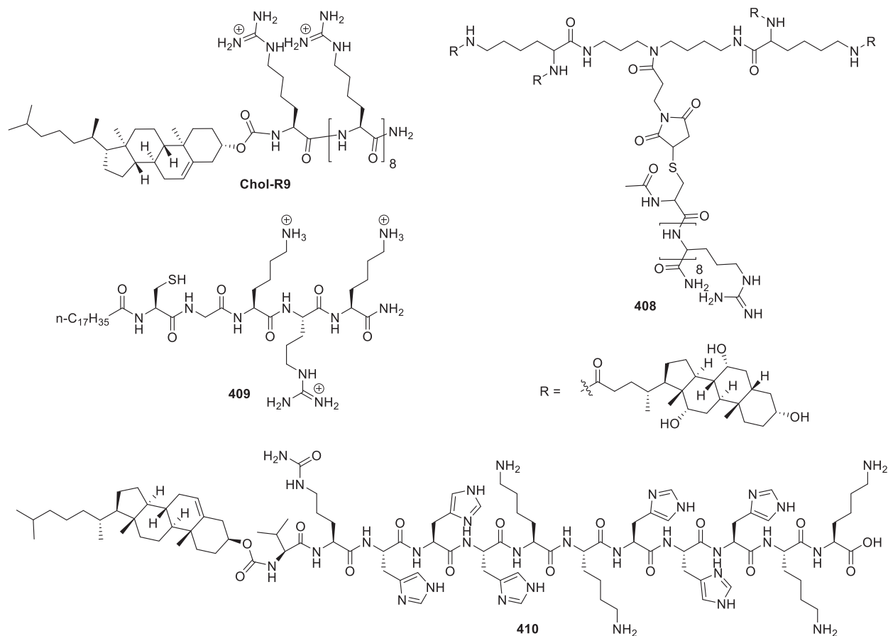
Figure 96. Chemical structures of lipopeptides.
