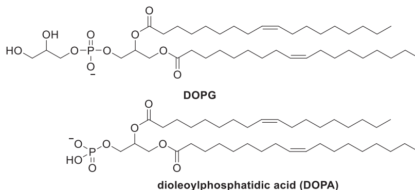
Figure 81. Chemical structures of representative phosphatidylglycerol.
