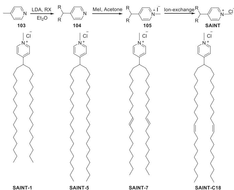
Figure 21. Chemical structure and synthesis of SAINT.
