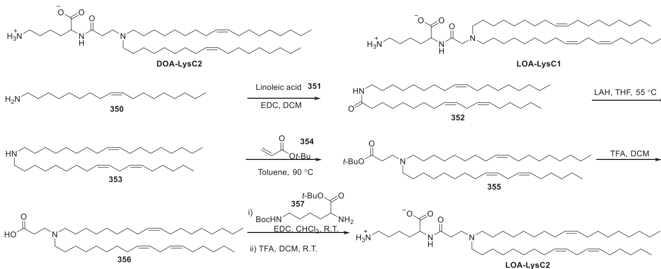
Figure 71. Chemical structures of lysine-derived zwitterionic lipids.
