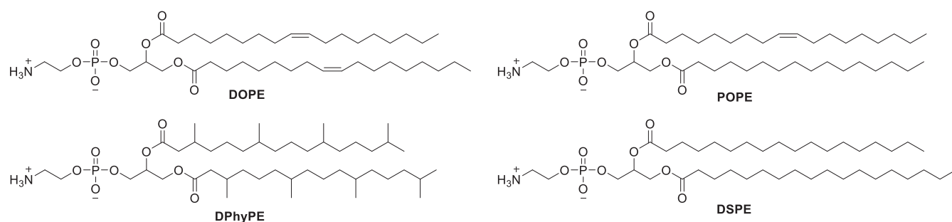
Figure 80. Chemical structures of representative phosphatidylethanolamines.
