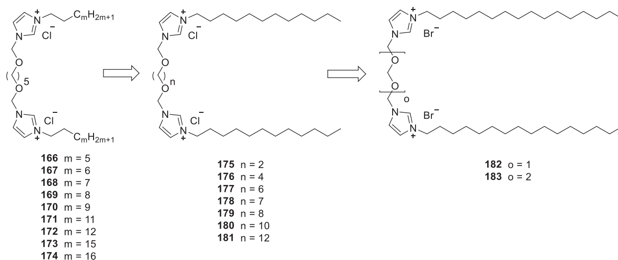
Figure 28. Optimization of imidazolium gemini surfactants.
