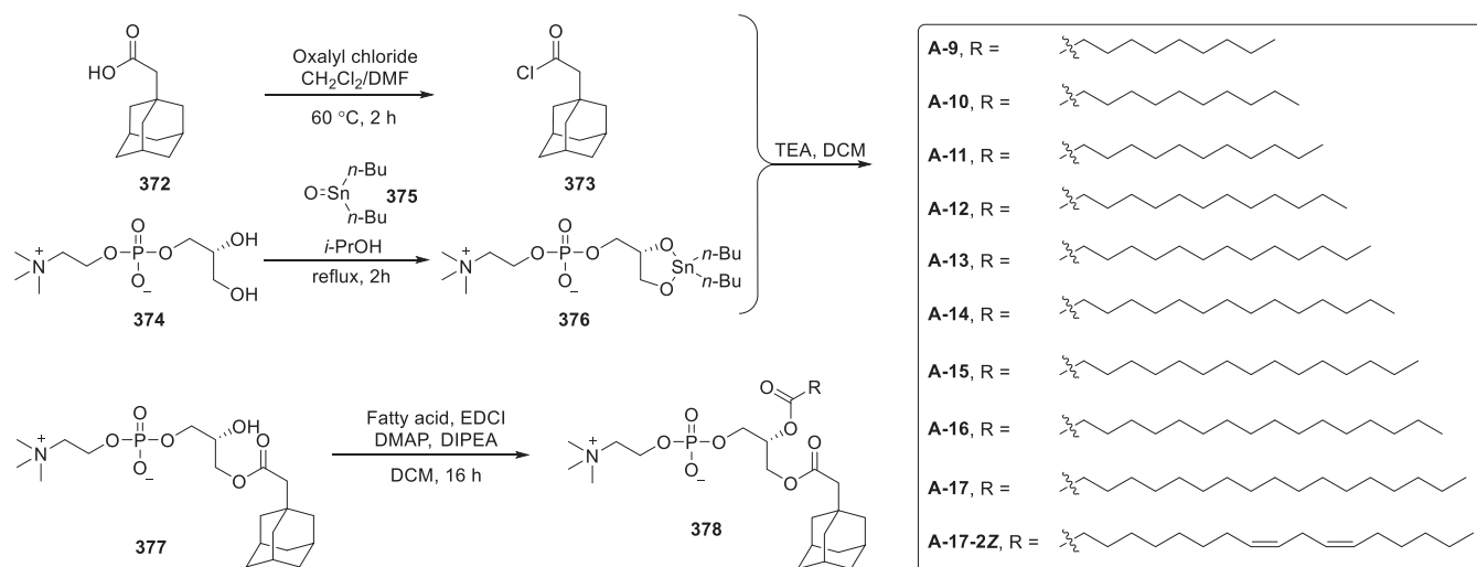
Figure 79. Synthesis of phosphatidylcholines incorporating adamantyl groups.
